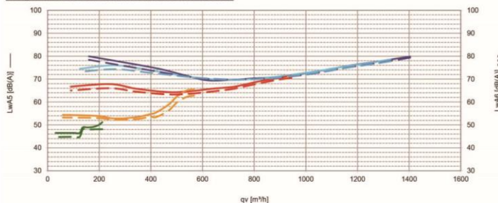
2. Diagramm / Chart - Volumenstrom - Akustik / Airflow - Acoustics
